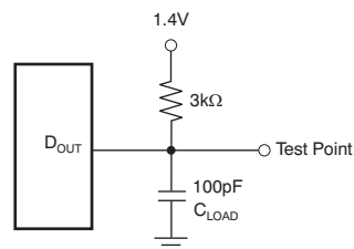
Load Circuit for t_{\text{dO}} , t_r , and t_f
