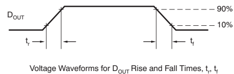
Voltage Waveforms for \text{D}_{\text{OUT}} Rise and Fall Times, t_r , t_f
